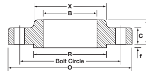
Slip-On Welding
