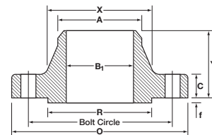
Welding Neck
