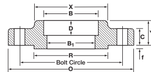
Socket Welding 1/2" - 2 1/2"
