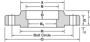
Socket Welding 1/2" - 3"
