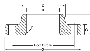
Lapped
