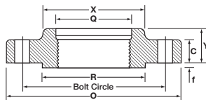
Threaded Class 300 - 2500
