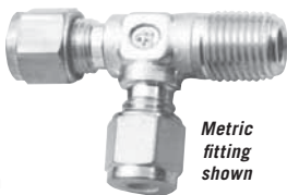
Dimensions — inches
