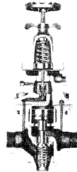
High Performance Air or Steam Bronze Body, Stainless Trim 600 PSI Max. Inlet Air 585 PSI Max. Outlet Air 300 PSI Max. Inlet Steam 275 PSI Max. Outlet Steam Threaded or Flanged Ends SIZES: 1/2" to 3"
