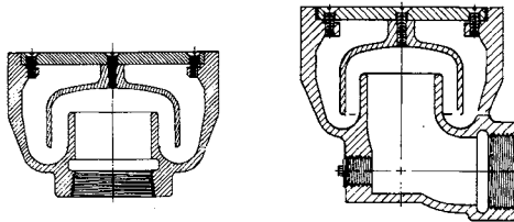
With Trap & Baffle Angle Type 511502 511602
