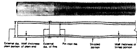
Integral Low Finned Tube
