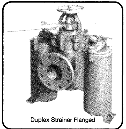
Duplex Strainer Flanged 150 LB Bronze 692501 150 LB Steel 692601 125 LB Iron 692600
