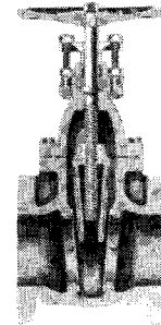
NRS Cutaway
