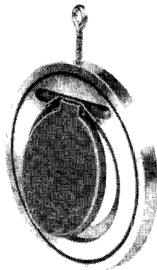
Thin Wafer Style Swing Check Steel 308101 Bronze 308502 Stainless 308707
