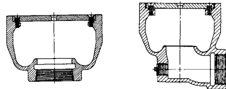
Without Trap & Baffle Angle Type 511501 511601
