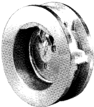
Wafer Swing Check Iron 305202 Steel 305101 Bronze 305503 Stainless 305707
