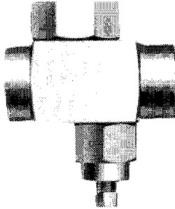
Thermodynamic TD-S-52 with Integral Strainer Max. Pressure 600 PSI / 800° F Threaded Ends Sizes 1/2" to 1" Fig. 531102 - Threaded
