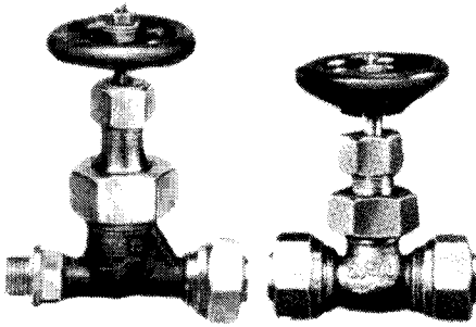
Male Thread by Union Socket 6 & 10 mm
