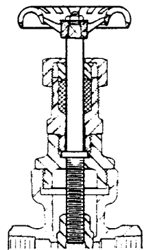
Inside Screw Non-Rising Stem
