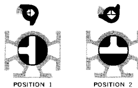
3 Way 3 Port Flow 5
