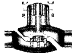
Piston Check Threaded 173607 Socketweld 173637
