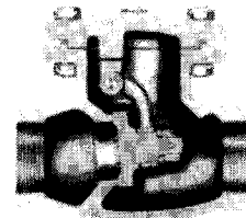
Swing Check Threaded 176507 Socketweld 176537
