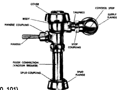
Typical Flush Valve
