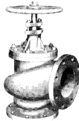
High Lift Cargo Angle
