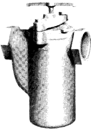
THREADED SIMPLEX BASKET STRAINER 150 LB Bronze - 691501 150 LB Steel - 691601 125 LB Iron - 691801
