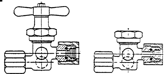
Globe - 418301 Angle - 418401 Check - 418601
