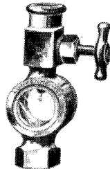
Sight Feed Valve Bronze Straight Heavy Pattern Sizes 1/4" to 1/2"
