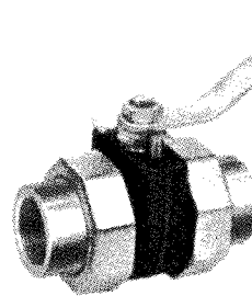
Union End Threaded, Socketweld or Silbraze Bronze Thrd 375502 Bronze S/B 375532 Steel Thrd 376501 Steel SW 376531 Stainless Thrd 377507 Stainless SW 377537
